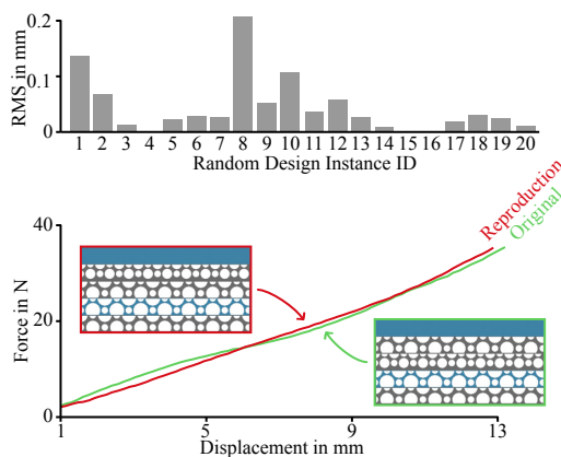
Figure 9: Validation of goal-based design algorithm. We randomly generate a set of material designs. We then simulate these designs and use their simulated deformations as the input to the goal-based design search algorithm. We then compare the obtained designs of the search algorithm with the known ground truth. The upper bar plot shows the RMS error. We also fabricated one of those randomly generated designs and its corresponding search output and compared their force-displacement curves.
